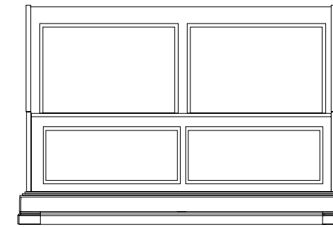
864-90-220 Sleigh Bed, 5/0 Queen 68 1/4W x 102 3/4D x 60 1/4H (173 x 261 x 153 cm) Consists of: 864-90-221 5/0 Sleigh Headboard 68 1/4W x 18 1/4D x 60 1/4H (173 x 46 x 153 cm) 864-90-222 5/0 Sleigh Footboard 67 3/4W x 7D x 33 3/4H (172 x 18 x 86 cm) 864-90-223 5/0 Sleigh Rails w/CSS 78W x 3 1/2D x 11 1/2H (198 x 9 x 29 cm)
